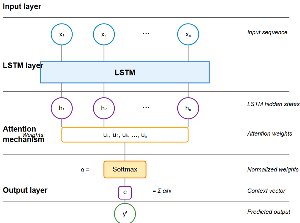
Figure 3. The Proposed LSTM-Attention Mechanism
