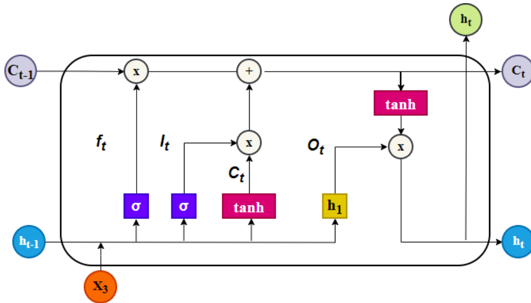
Figure 1. LSTM Neural Network Mechanism
