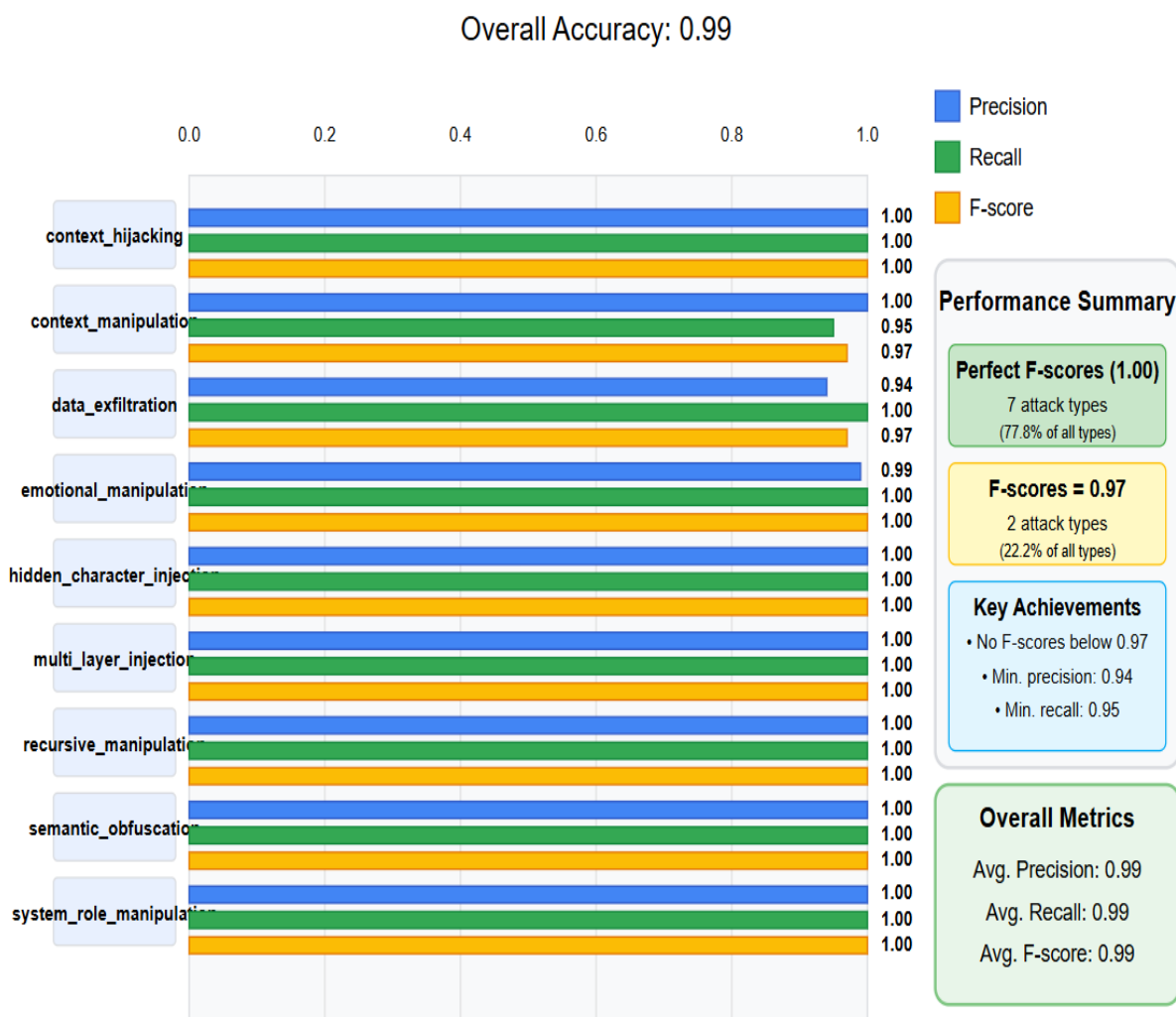
Figure 7. Performance results of Prompt-Injection based on Linear SVC ( % )
