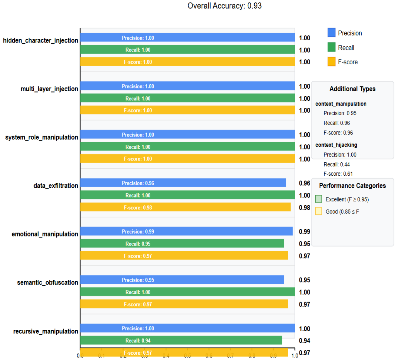
Figure 5. Performance results of Prompt-Injection based on k-NN Classifier ( % )
