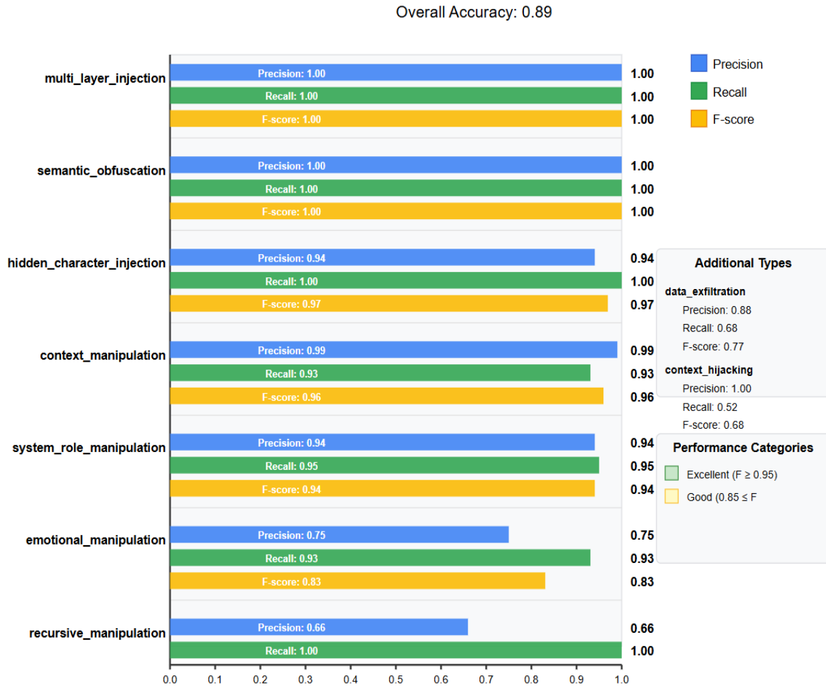
Figure 4. Performance results of Prompt-Injection based on Naive Bayes Classifier ( % )
