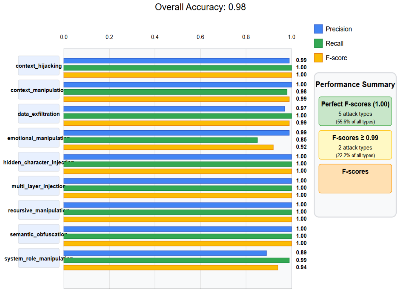
Figure 6. Performance results of Prompt-Injection based on Random Forest ( % )
